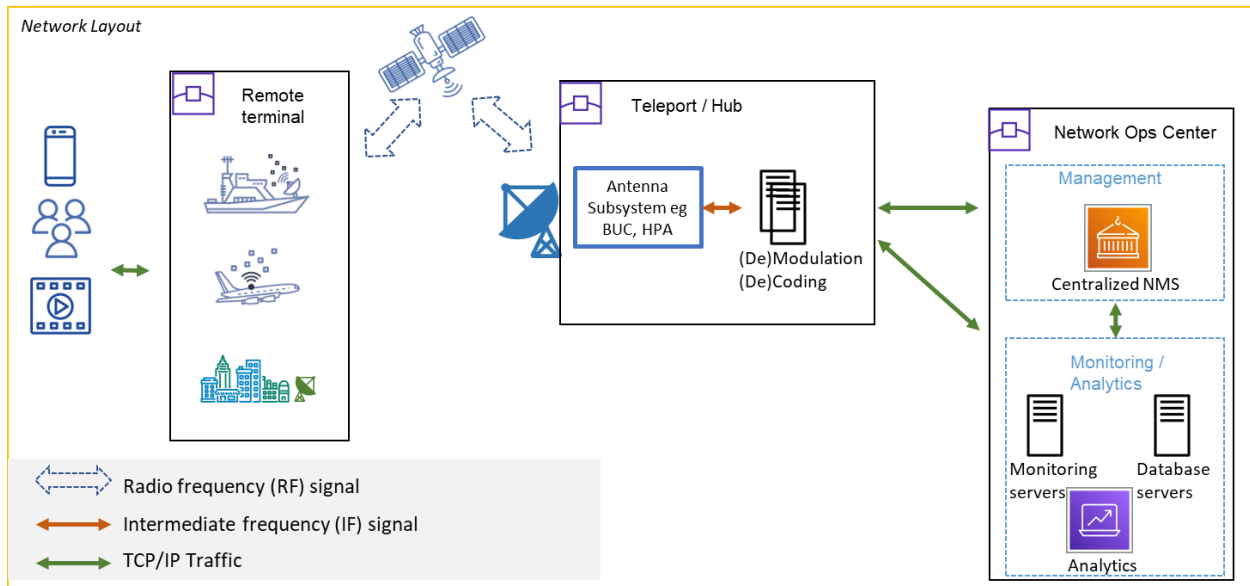
Fig. 1: Architectural diagram of a traditional satellite communications system
