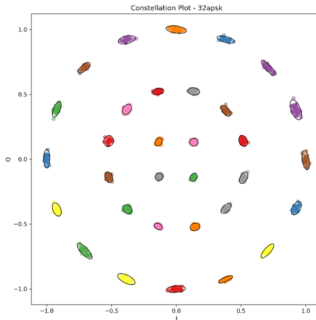
Fig. 4: Phase noise impairment of a 32APSK constellation
