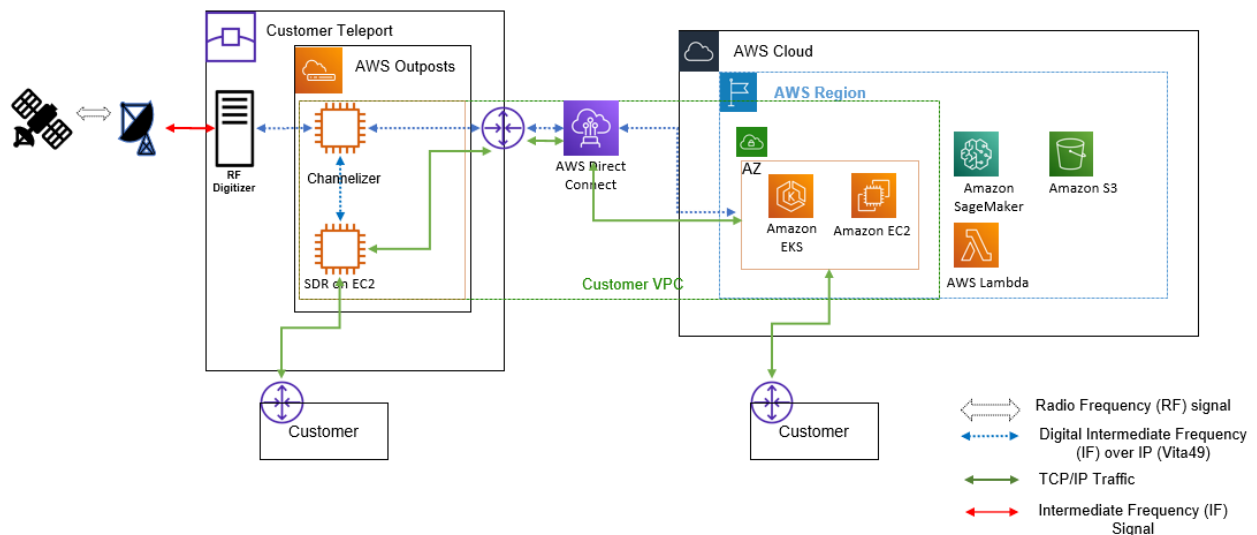
Fig. 2: Architectural diagram of a virtualized satcom system with SDR (de)modulation, (de)coding in AWS Cloud
