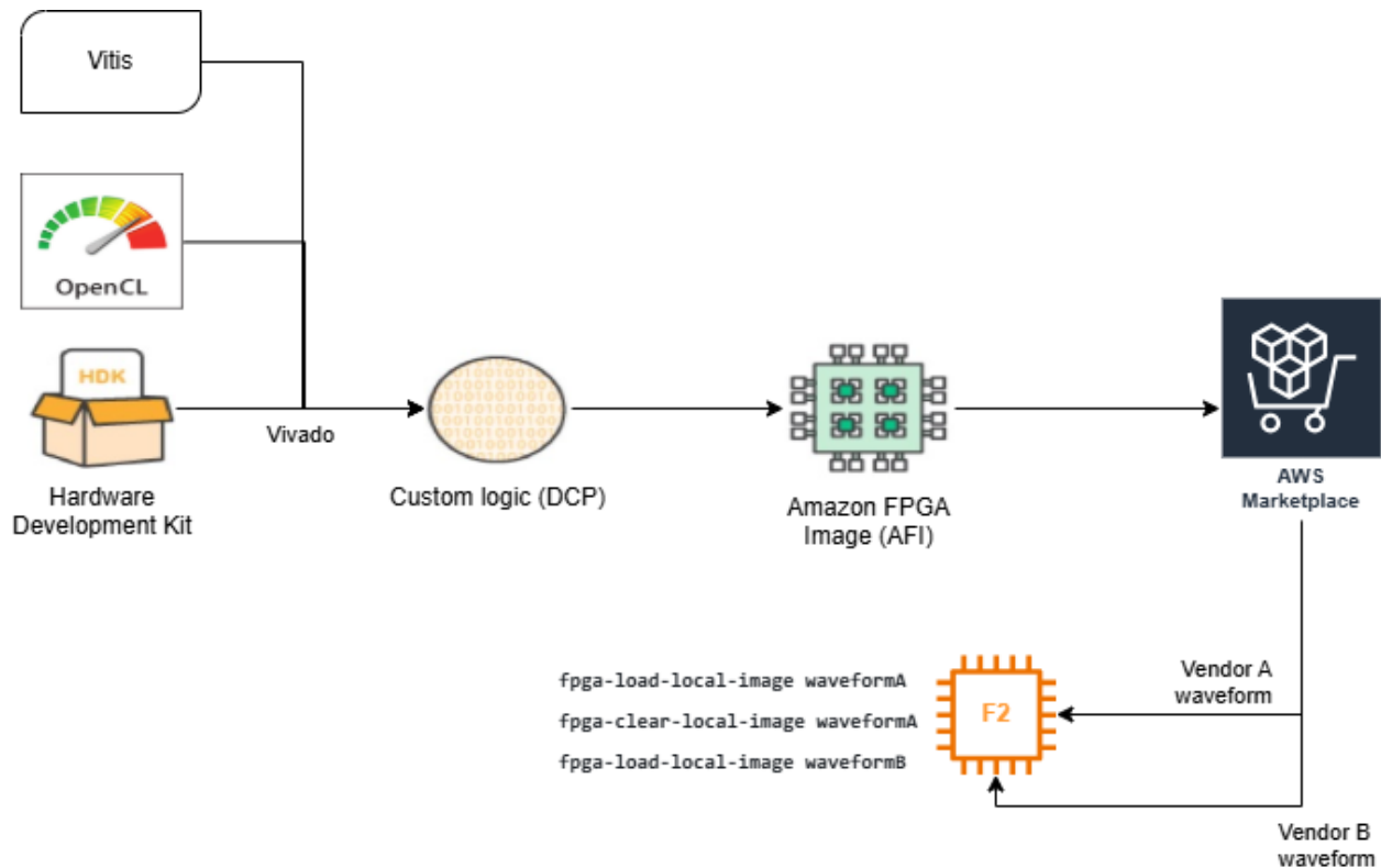
Fig. 3: Waveform orchestration with EC2 F2 FPGA
